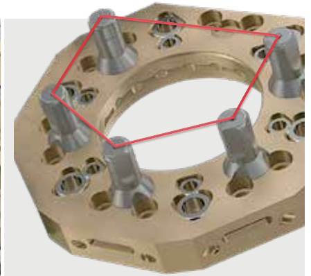
Exact fusion due to conical guide columns
